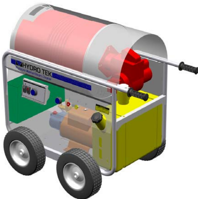
HP Ultimate Series Front view with optional wheel kit
